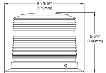
Low Dome
